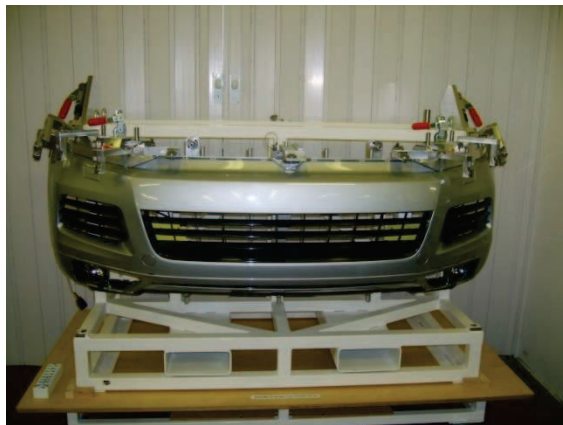
Bumpers Checking Fixtures
