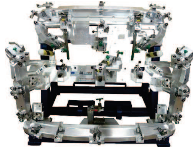
Tailgate Checking Fixture
